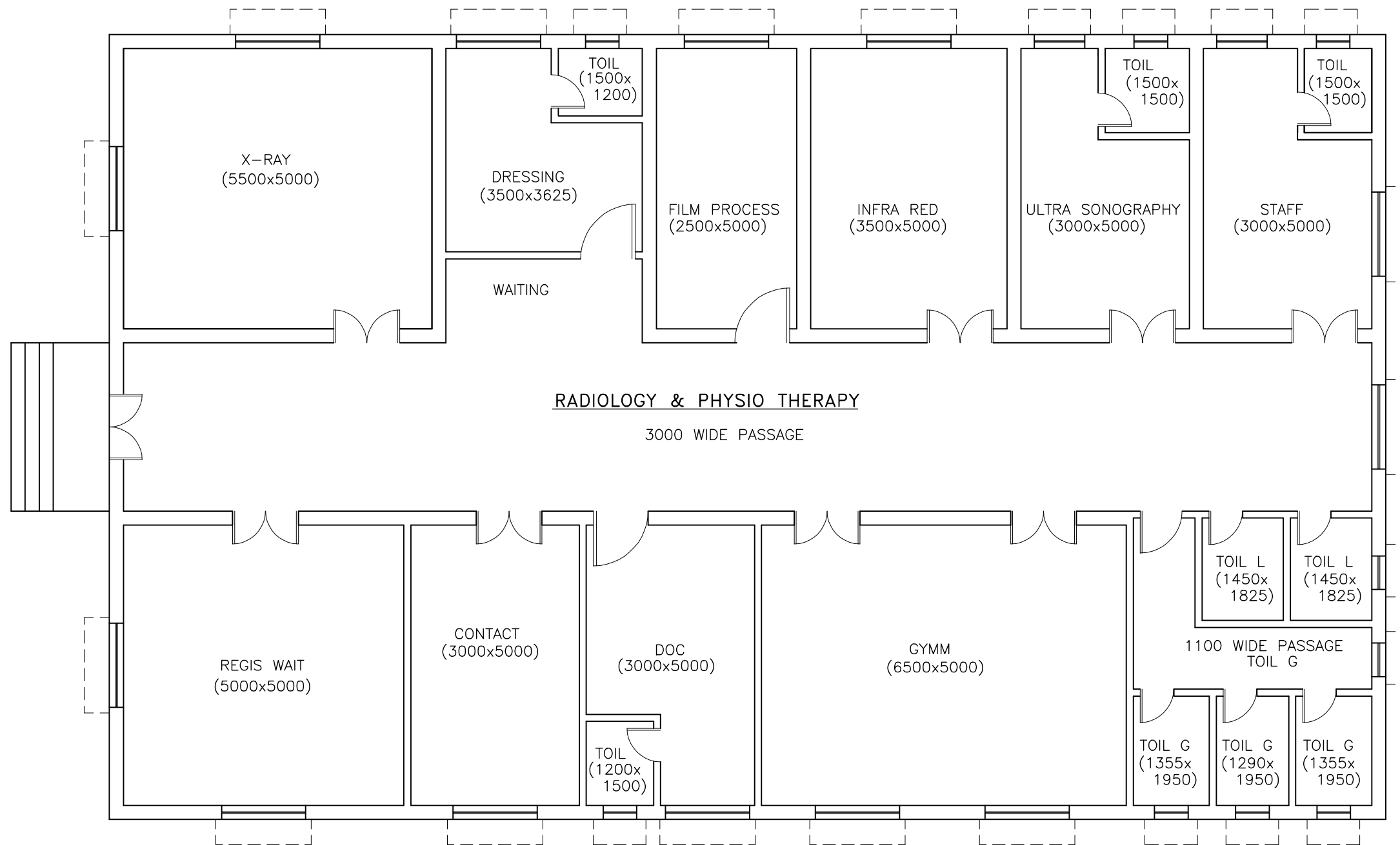
PLAN OF RADIOLOGY & PHYSIO THERAPY DEPARTMENT
